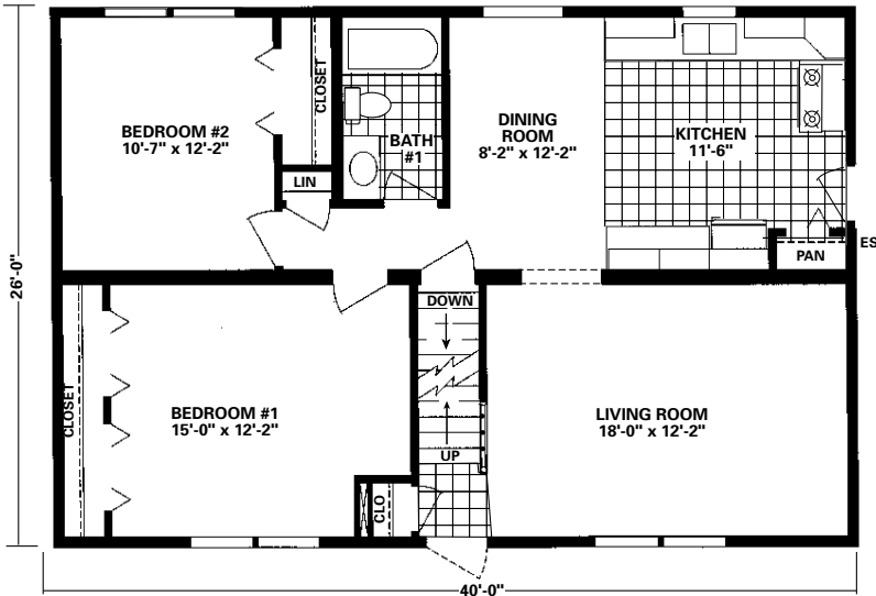
4426-112 1144 Sq. Ft. - LOWER LEVEL
