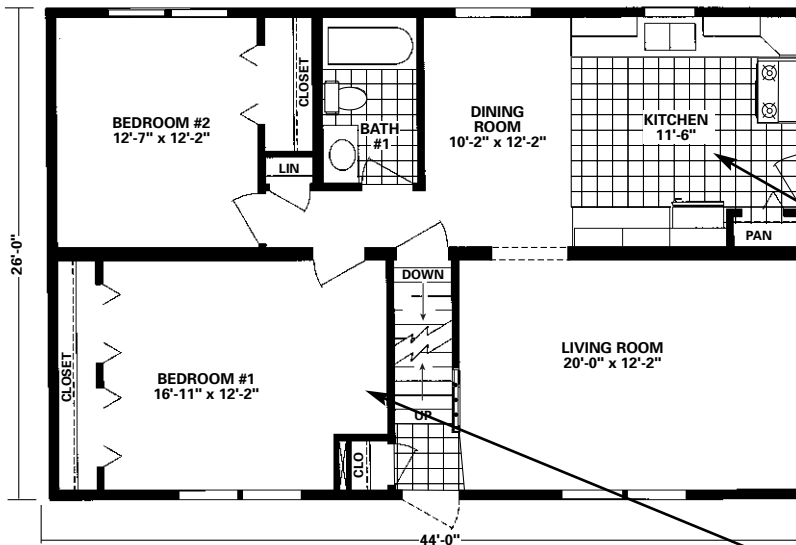
4426-112 1144 Sq. Ft. - LOWER LEVEL
